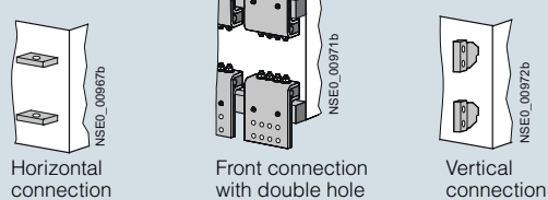
Main circuit connections
